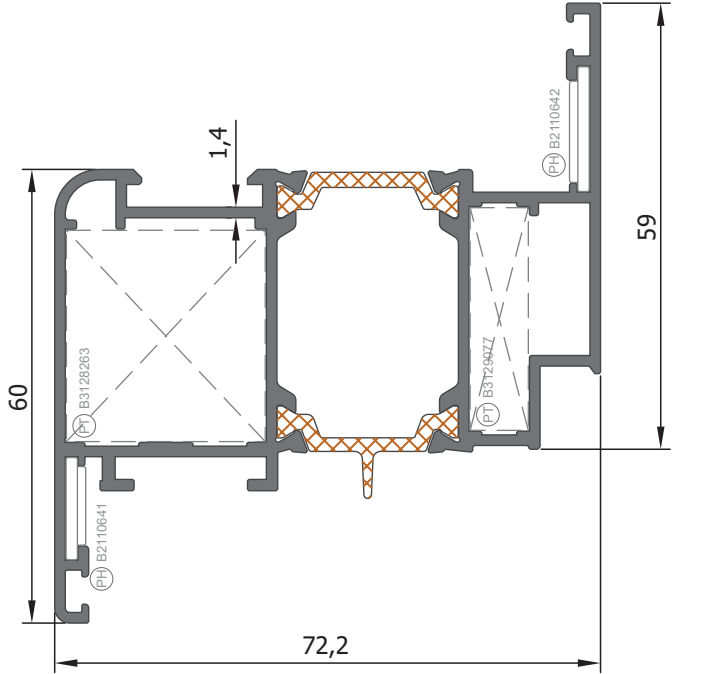
Kanat Profili 1.4 mm. Sash Profile
