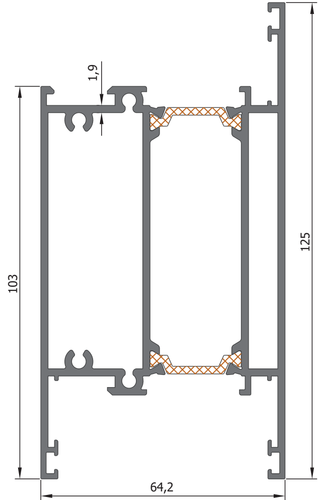
Kanat Profili 1.9 mm. Sash Profile
