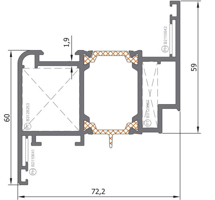
Kanat Profili 1.9 mm. Sash Profile
