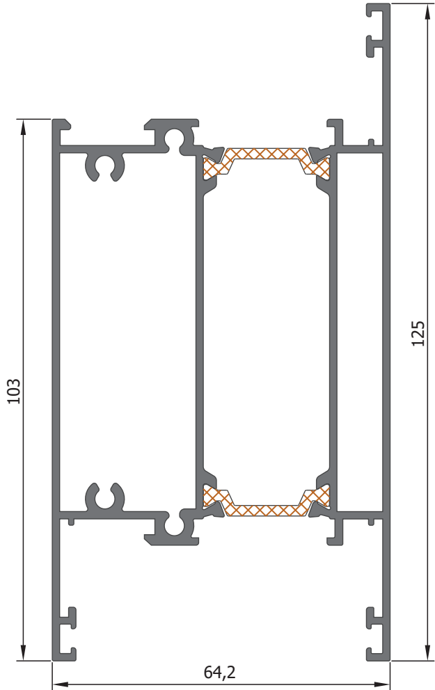
Kanat Profili 1.4 mm. Sash Profile
